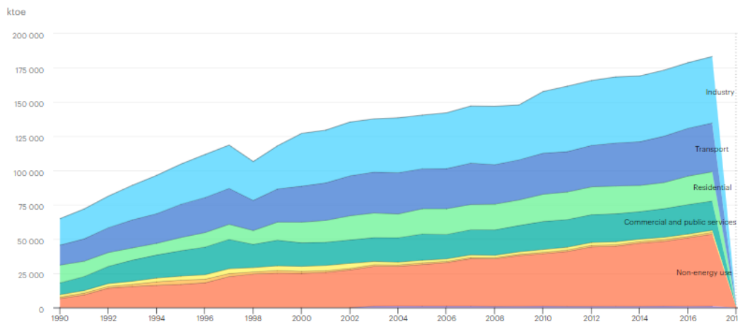
Total final consumption (TFC) by sector, Korea 1990-2018
